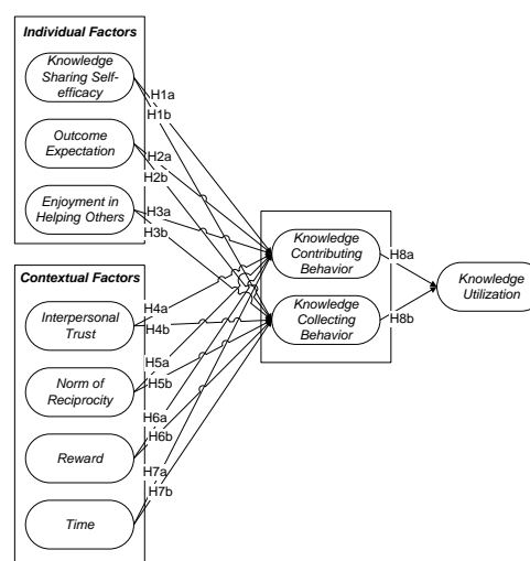
Figure1. Research model
