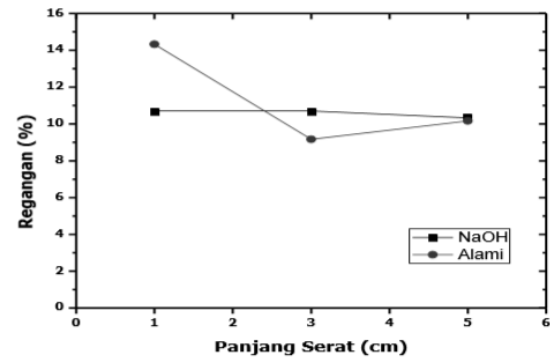
Figure 6. The Relationship between the strain agave fiber composite against the length of the fiber
